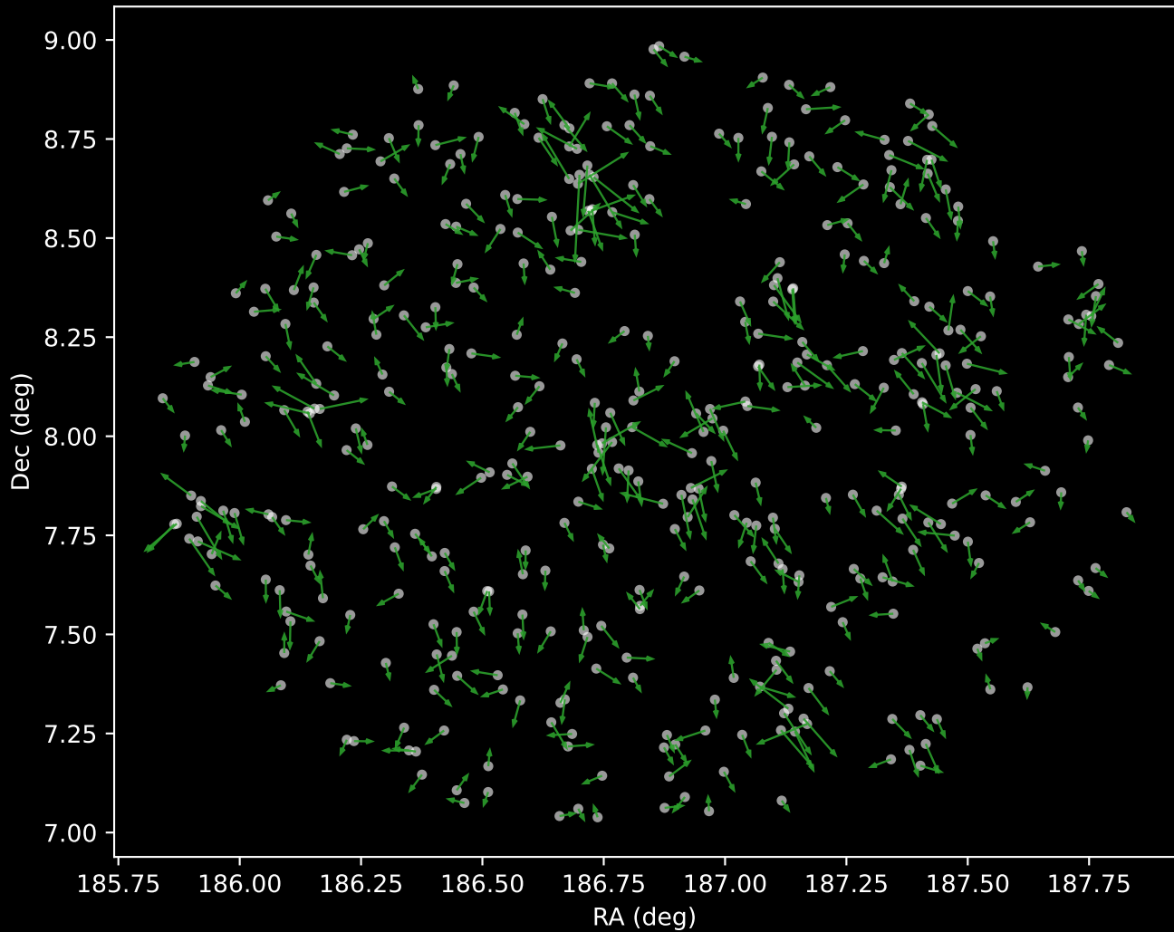
GALAH DR4 Cluster 4 Proper Motion Vectors (n=421)
