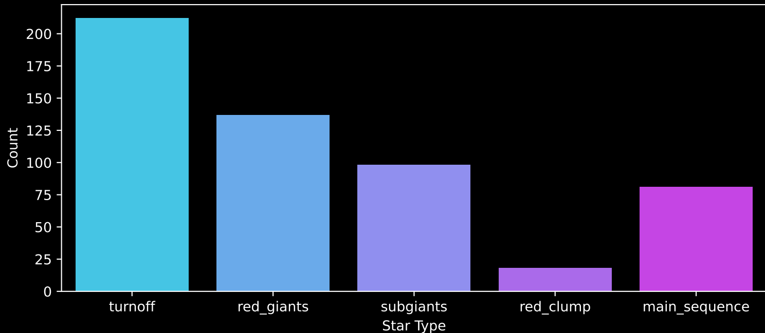
GALAH DR4 Field: [9466] Count plot of Star Type
