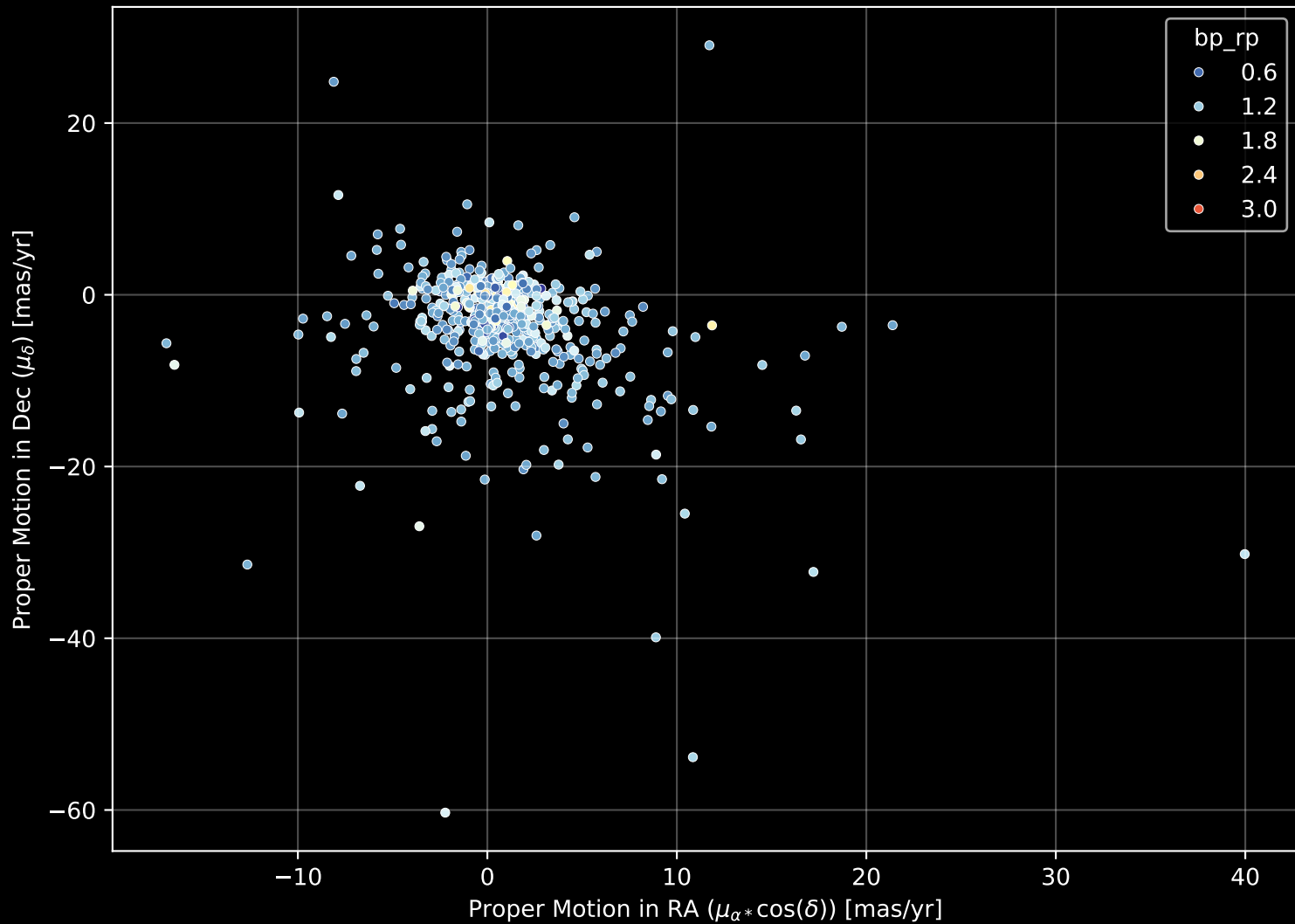
GALAH DR4 Field: [9466] Proper Motion Diagram (n= 546)
