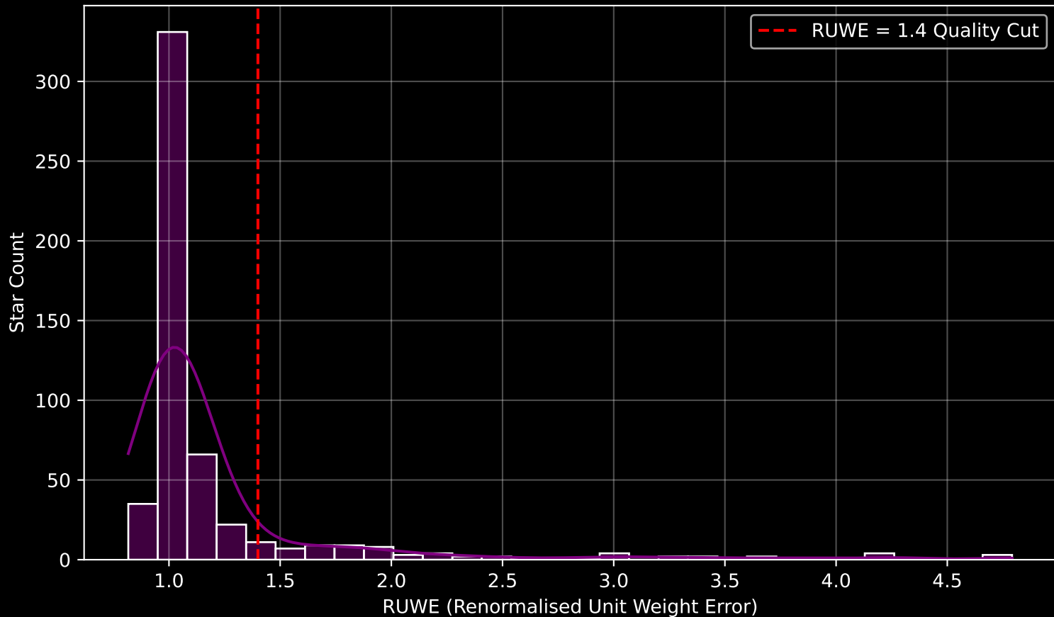
GALAH DR4 Field [9466] RUWE Distribution (n= 530)
